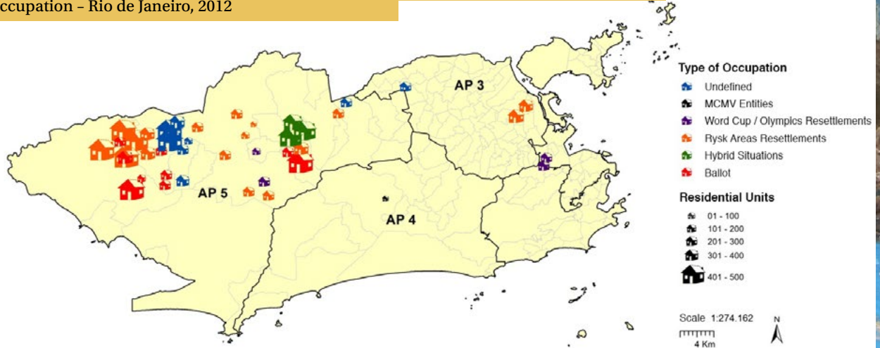
Map 1.1. Location of Minha Casa, Minha Vida developments by size of development and type of occupation - Rio de Janeiro, 2012
